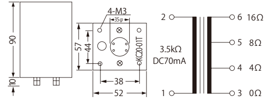
KC20-01T
