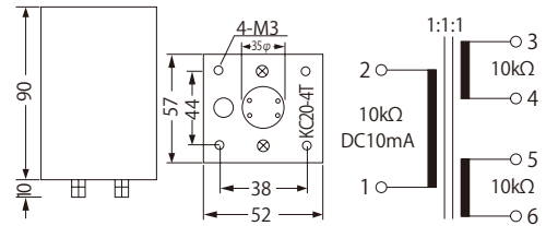
KC20-4T
