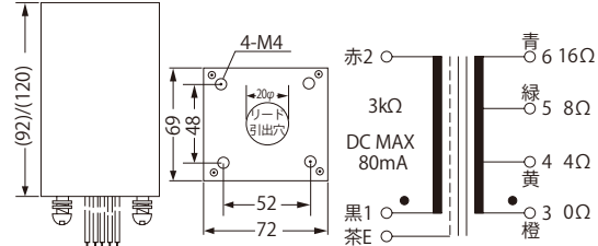
ASTR-01OPT
