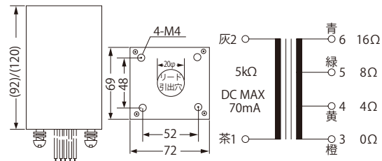
ASTR-02OPT
