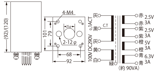
ASTR-03
